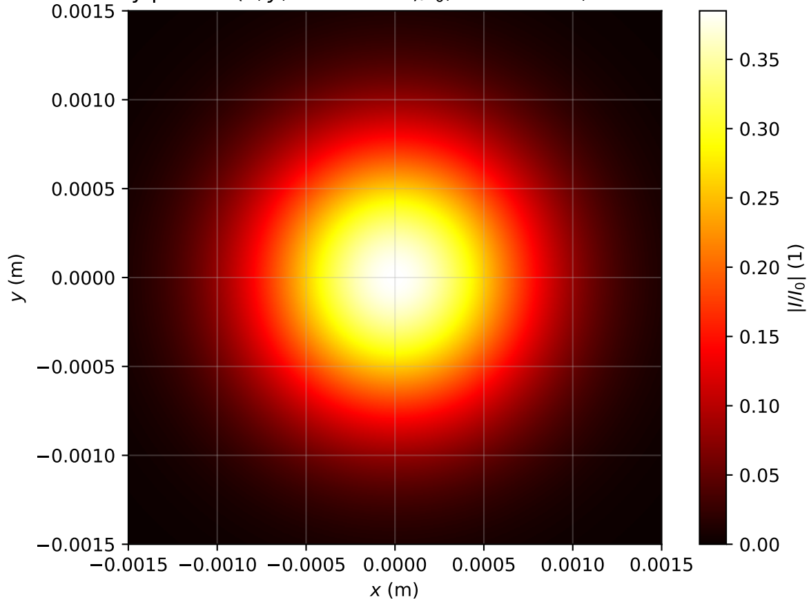
Intensity profile I(x, y, z = 2.707m)/I_0 , P_{in}=0.1P_{cr} , artificial time
